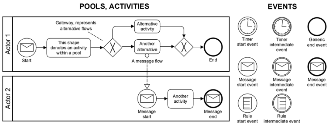
Figure 6: Key for interpreting the symbols used in the BPMN diagrams shown in Figures 4 and 5.
