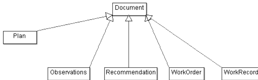
Figure 11: UML Class Diagram showing the class hierarchy of the Core Documents in ADAPT (AgGateway, 2016.)
