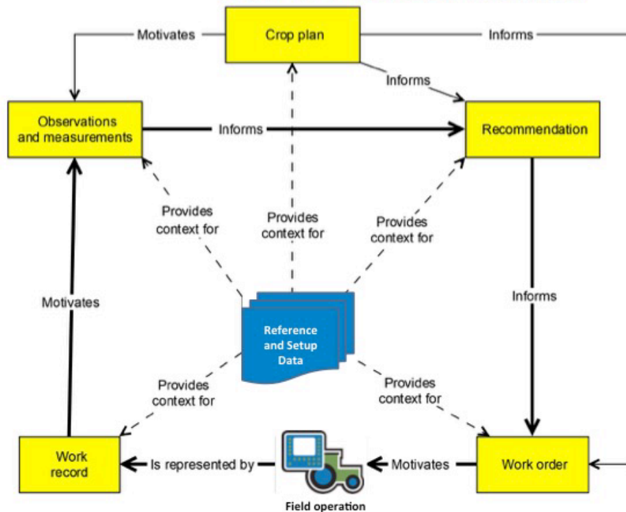
Figure 2. AgGateway Core Documents for Field Operations and the relationships among them,
