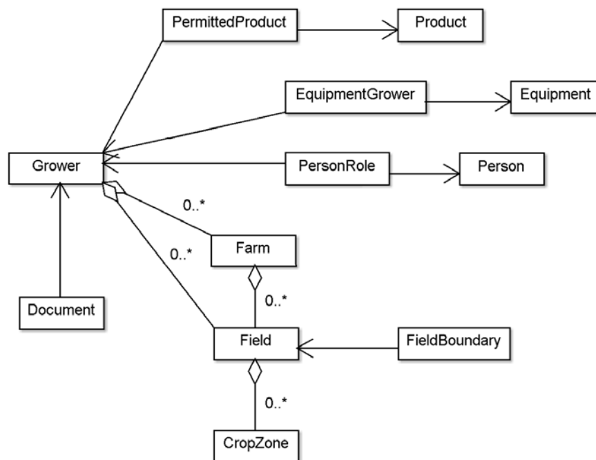
Figure 10: UML Class diagram showing PAIL implementation of Grower (Setup) Data.
