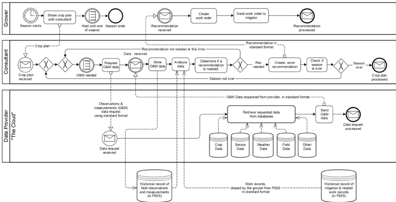
Figure 5: BPMN diagram showing Observations business process model.
