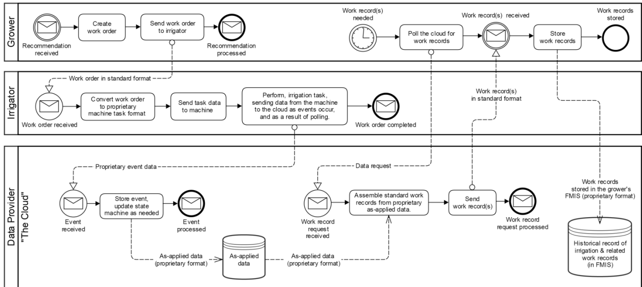
Figure 4: BPMN diagram showing Operations business process model.
