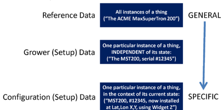
Figure 9: Reference, Setup, and Configuration Data
