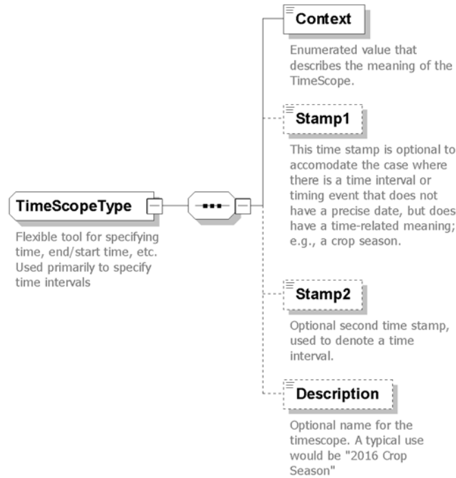
Figure 8: Representing time in the PAIL schema, with the TimeScopeType, a subset of the data available in ADAPT’s TimeScope class.
