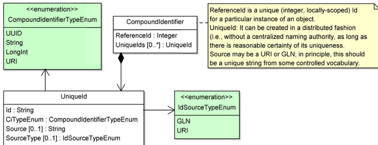
Figure 7: The CompoundIdentifier and UniqueId classes and their supporting enumerated vocabularies.
